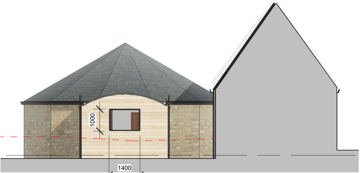
WEST ELEVATION - AS PROPOSED
